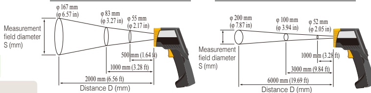
FT3700-20 Measurement distance and field diameter
