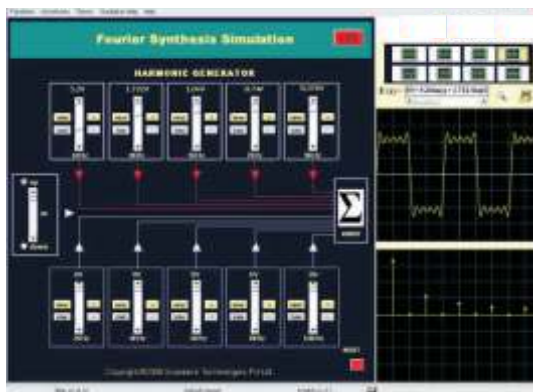
Software Results
